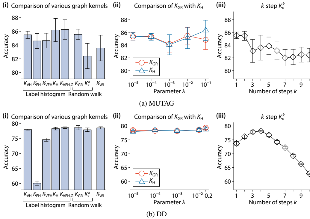
Figure S1: Accuracy results in real-world datasets (Means \pm SD).
