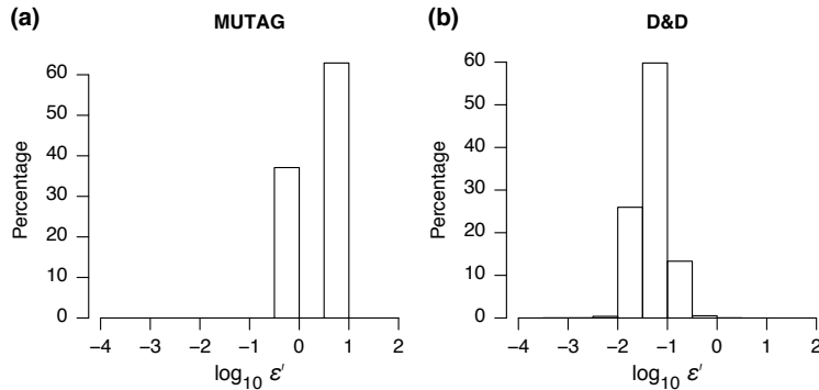
Figure S2: Distribution of \log_{10} \epsilon' , where \epsilon' is defined in Corollary 1, in real-world datasets.
